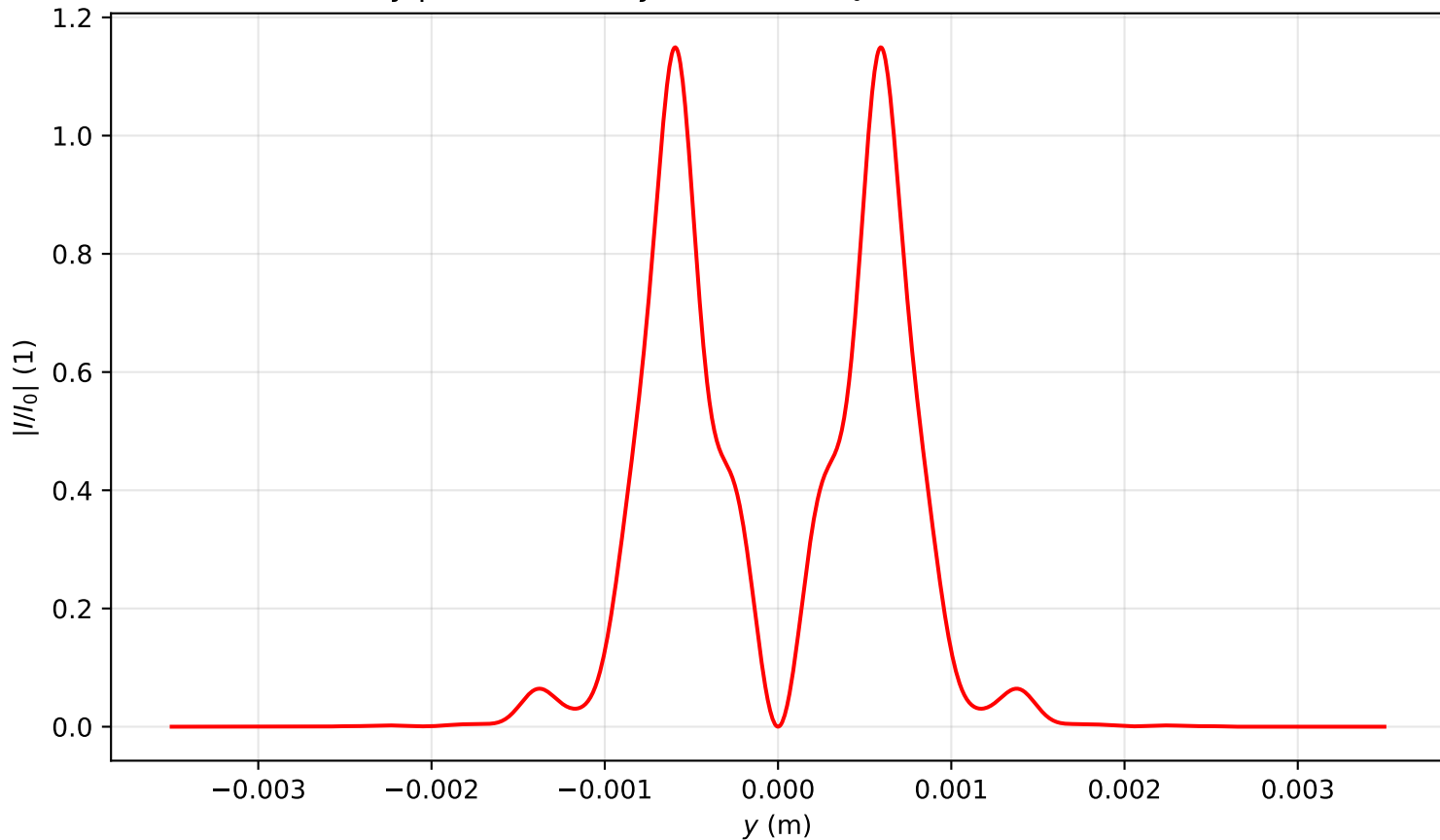
Intensity profile I(x=0, y, z=1.353)/I_0 , P_{in}=7.0P_{cr} , artificial time
